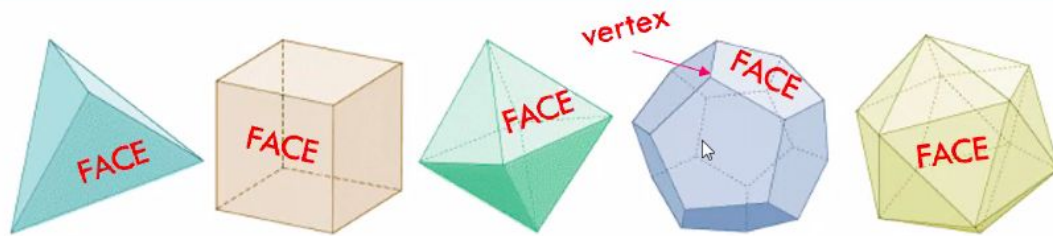
Tetrahedron
